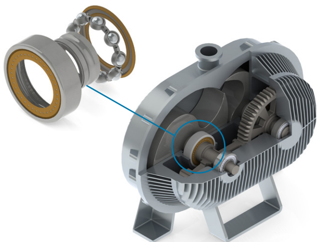
Claw Pump
