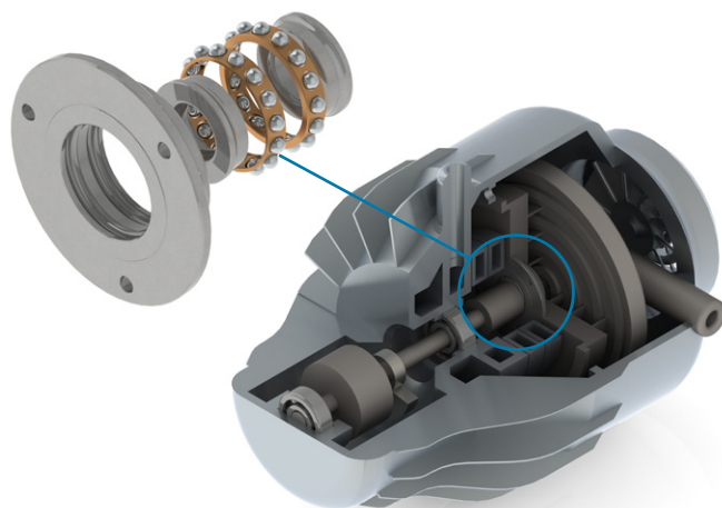
Scroll Pump
