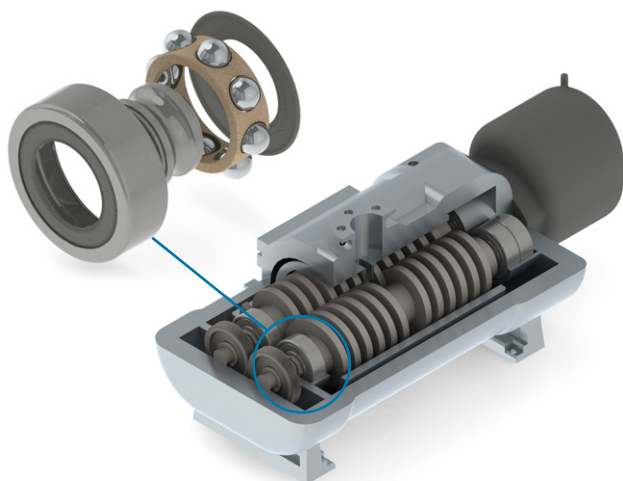
Screw Pump
