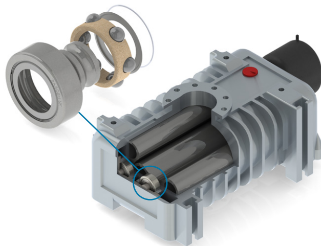
Roots Pump
