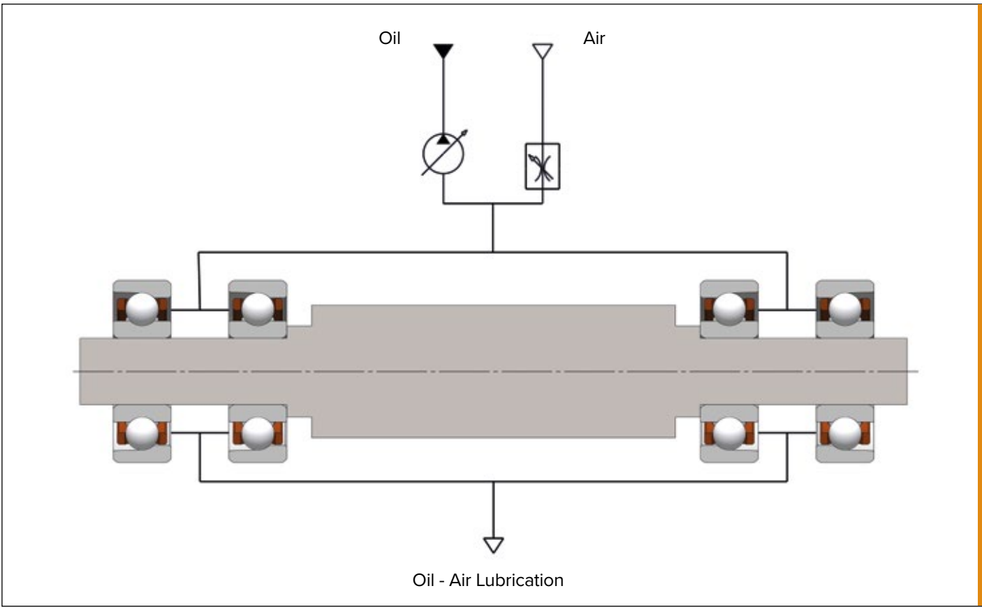
Oil minimum quantity lubrication (MQL)
