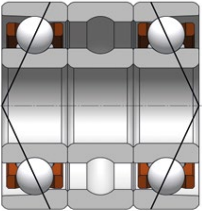
Bearing inner and outer ring as spacer
