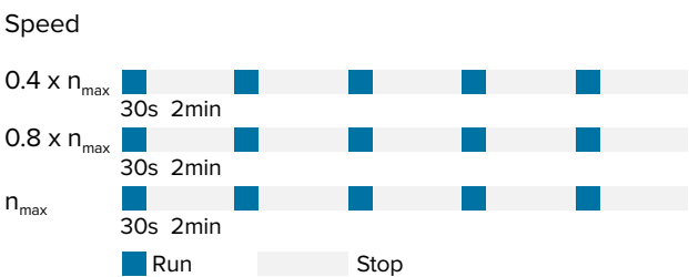
Grease distribution
